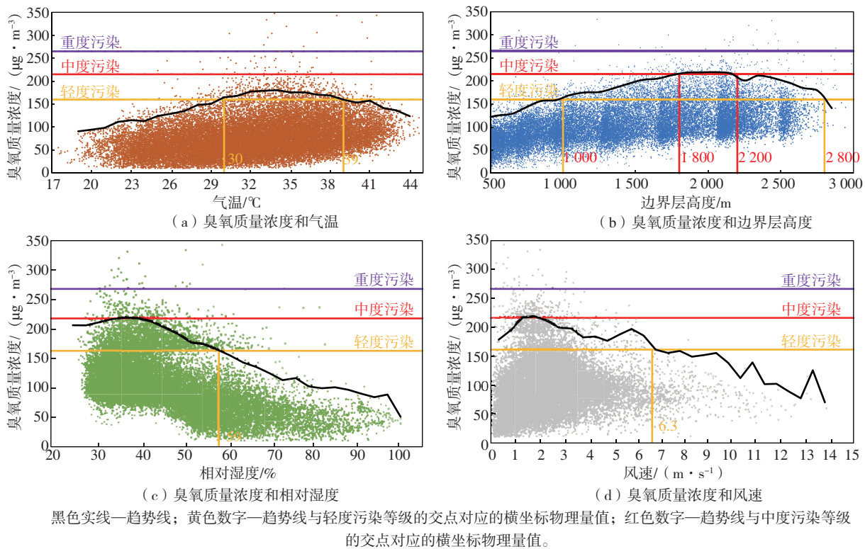
图6 7月1日—8月31日(08—20时)臭氧质量浓度和气象条件散点图 Fig.6 Scatter diagram of mass concentration of ozone and meteorological conditions between 08:00 and 20:00 from 1 July to 31 August
