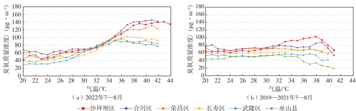
图7 重庆6个代表县(区)臭氧在不同气温下的平均质量浓度变化 Fig.7 Changes of average mass concentration of ozone under different temperatures in 6 representative counties (districts) of Chongqing
