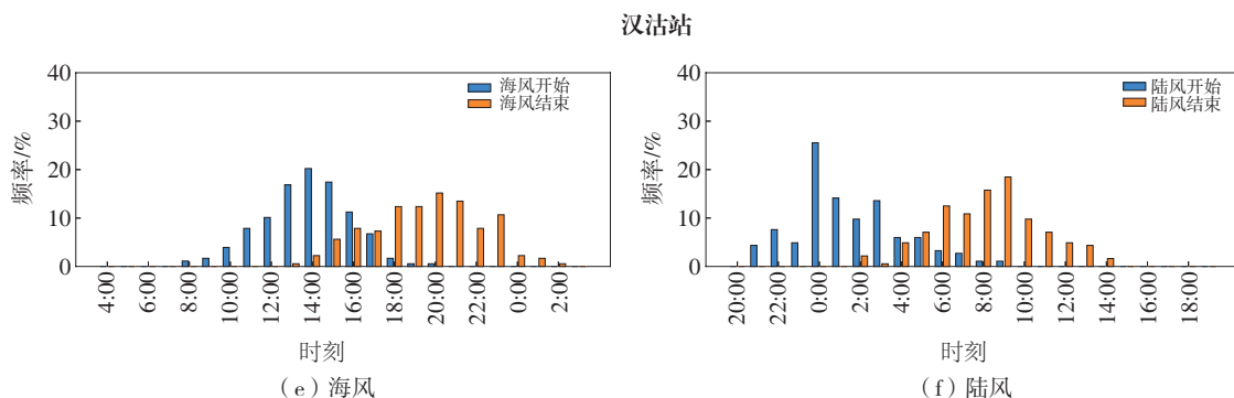
图3 站点资料显示的海陆风开始和结束时间的发生频率 Fig.3 Frequency of starting time and ending time of sea/land breeze revealed by observation data
