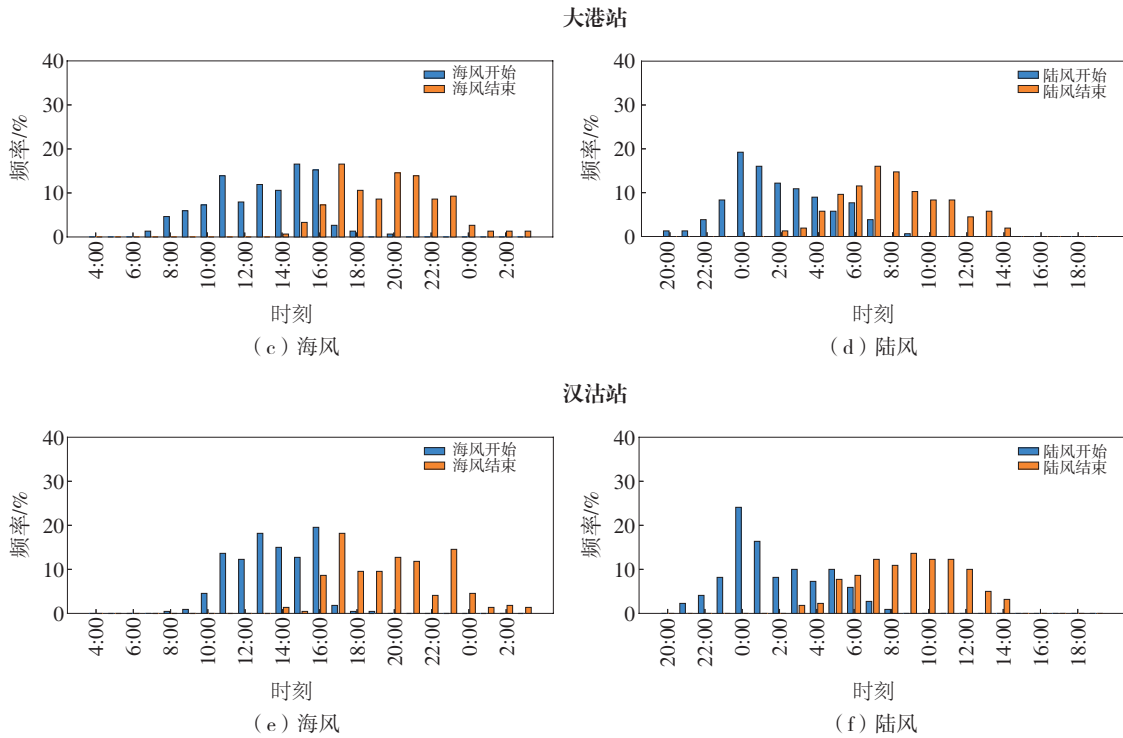
图 2 ERA5 资料显示的海陆风开始和结束时间的发生频率 Fig.2 Frequency of starting time and ending time of sea/land breeze revealed by ERA5
