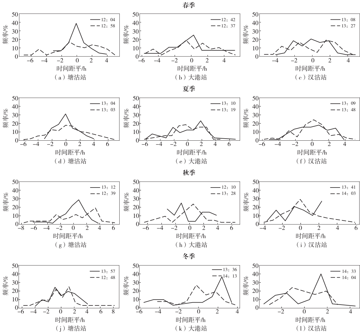
Fig.5 Comparison of sea-land breeze days at each station in each season by ERA5 and observation data
